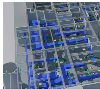
Subway Station MEP
